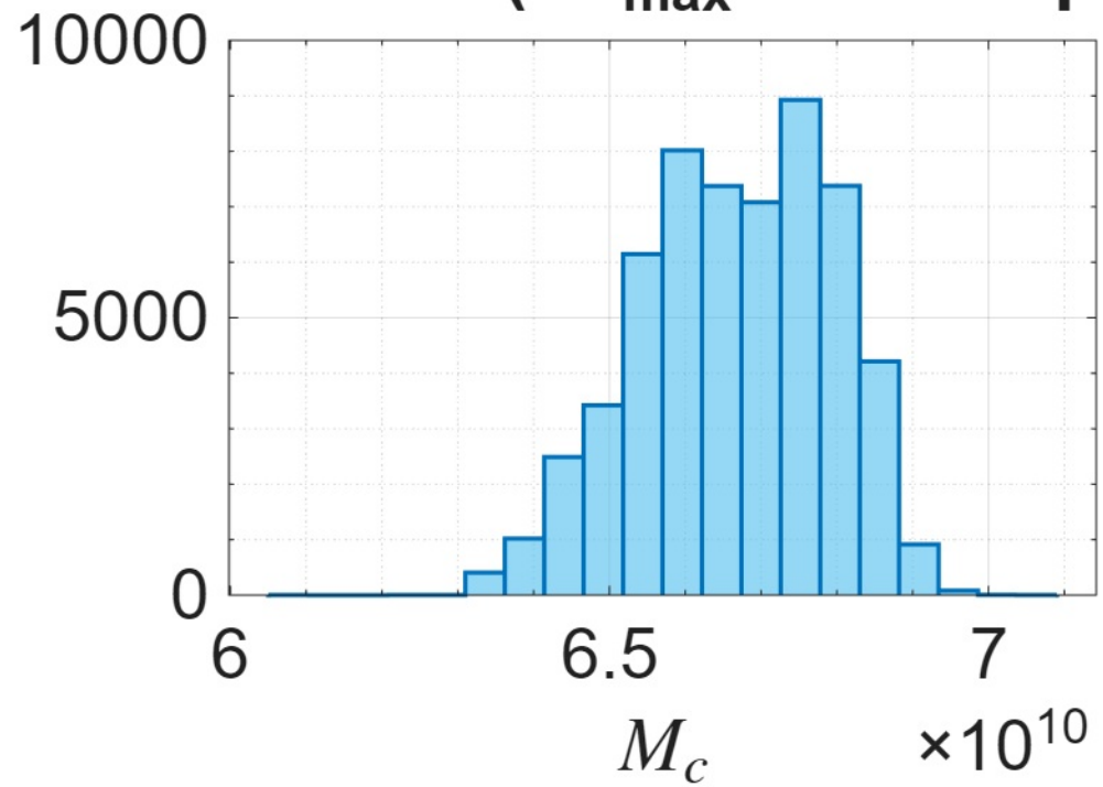
NGC0247 ( R_{\text{max}} = 14.54\text{kpc} )
