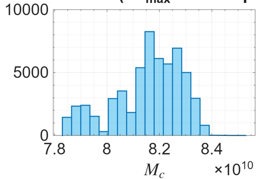
NGC0891 ( R_{\text{max}} = 17.11\text{kpc} )
