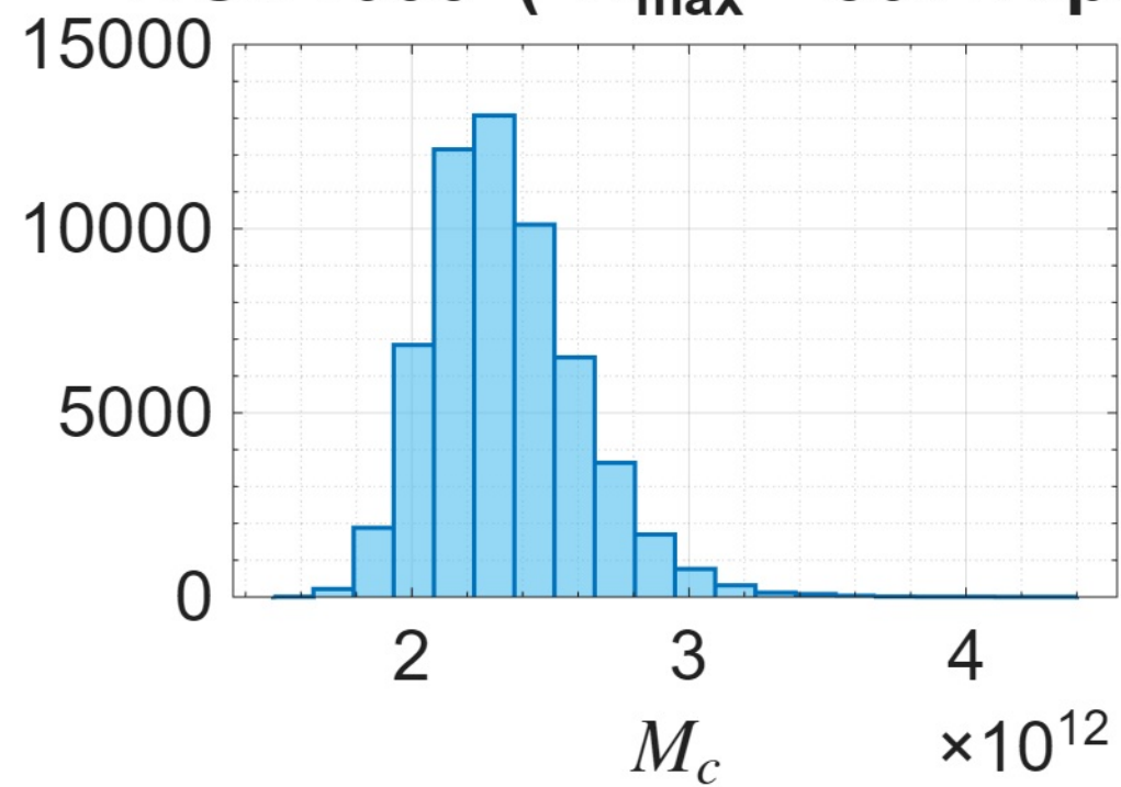
NGC1003 ( R_{\text{max}} = 30.24\text{kpc} )
