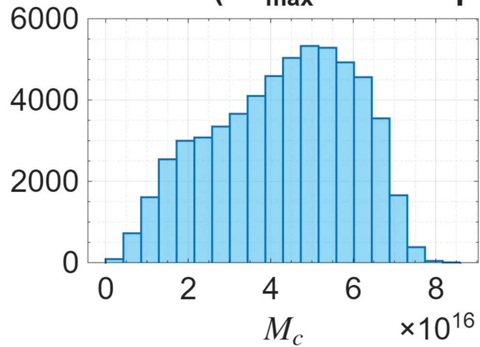
NGC1090 ( R_{\text{max}} = 30.09\text{kpc} )
