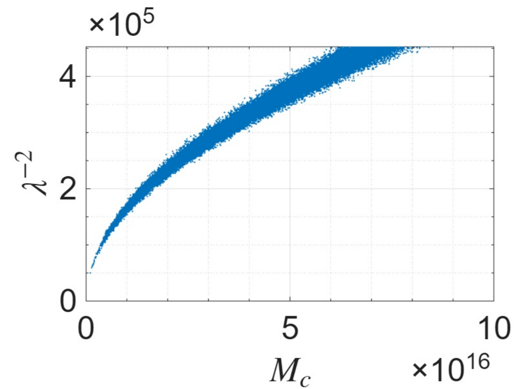
NGC1090 ( R_{\text{max}} = 30.09\text{kpc} )
