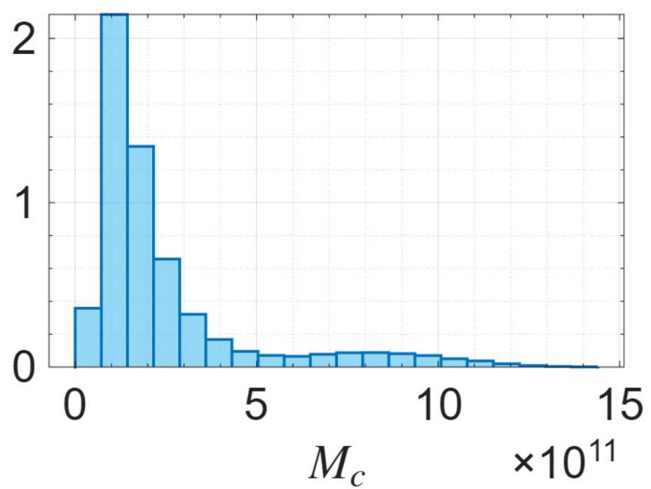
NGC1705 ( R_{\text{max}} = 6\text{kpc} )
