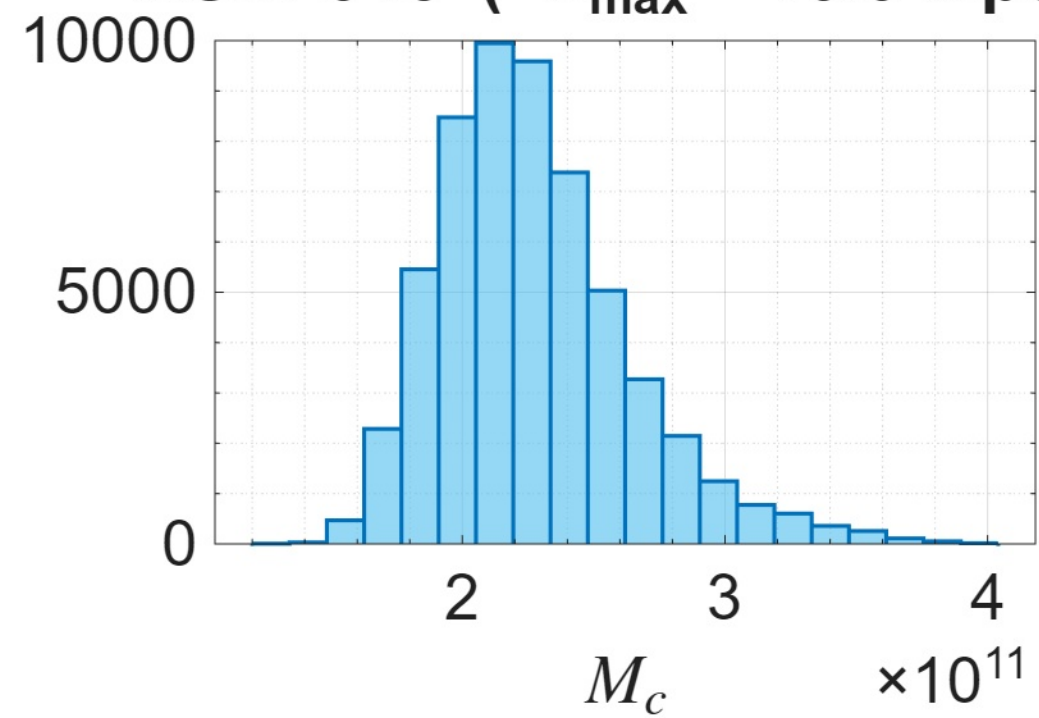
NGC2915 ( R_{\text{max}} = 10.04\text{kpc} )
