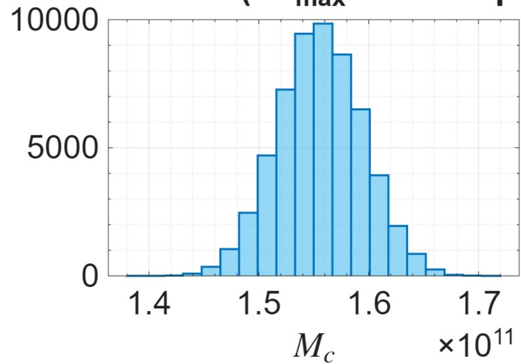
NGC2955 ( R_{\text{max}} = 35.43\text{kpc} )
