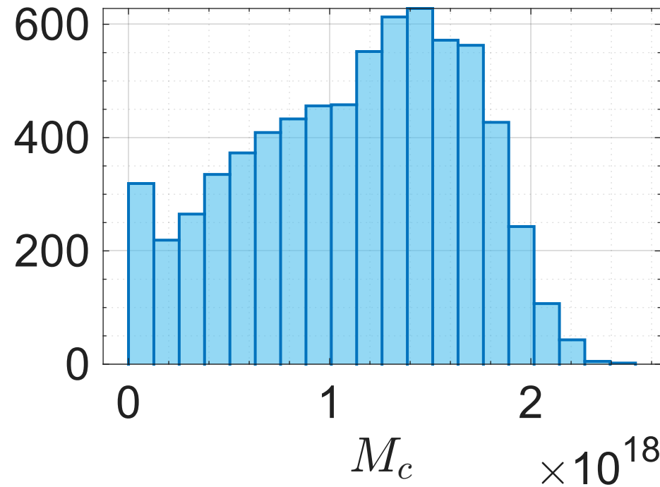
UGC02885 ( R_{\text{max}} = 74.07 \text{kpc} )
