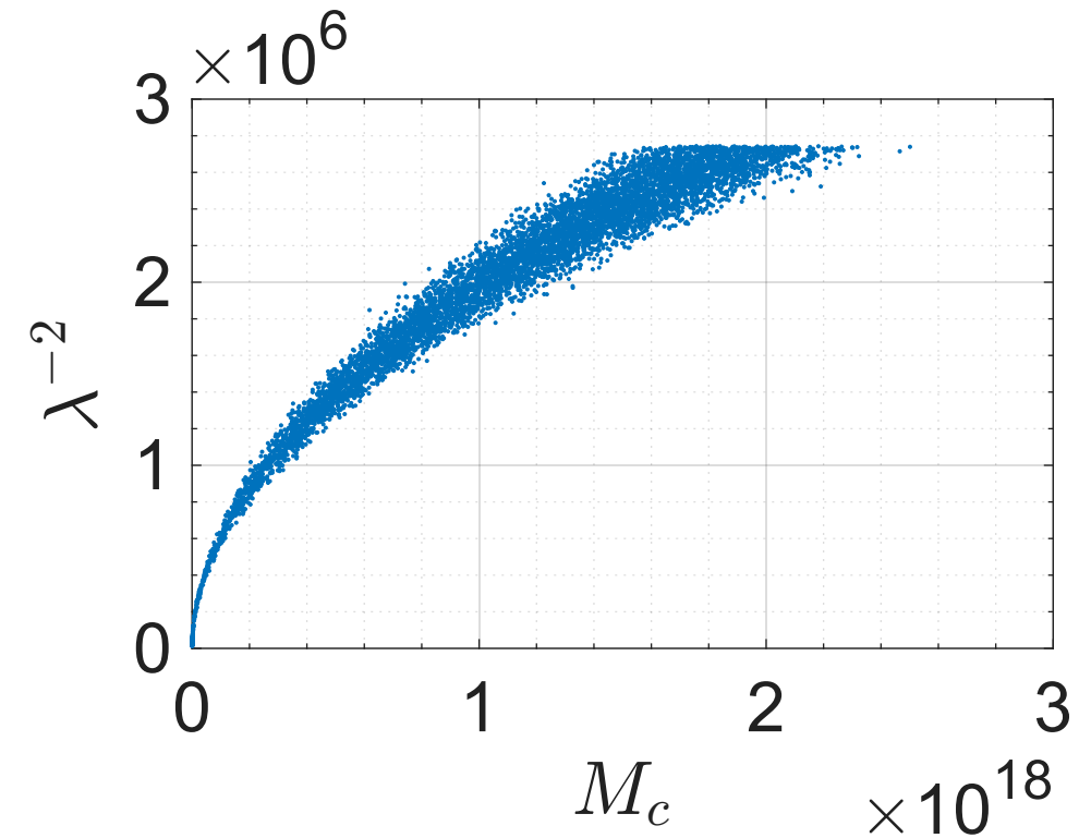
UGC02885 ( R_{\text{max}} = 74.07 \text{kpc} )
