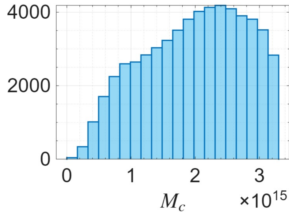
D631-7 ( R_{\text{max}} = 7.19\text{kpc} )
