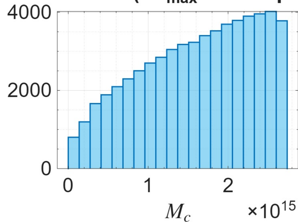
DDO064 ( R_{\text{max}} = 2.98\text{kpc} )
