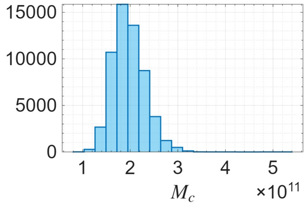
F563-V2 ( R_{\text{max}} = 10.47\text{kpc} )
