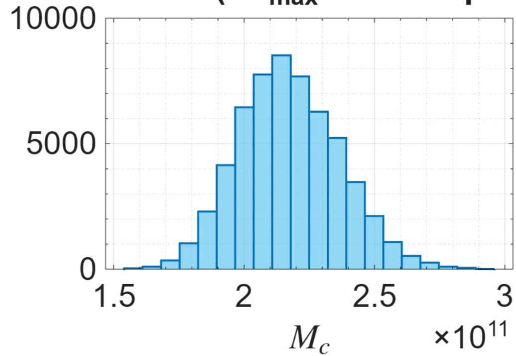
F583-1 ( R_{\text{max}} = 16.26\text{kpc} )
