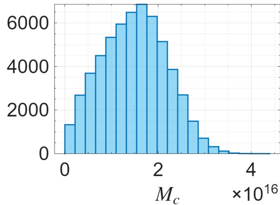
IC4202 ( R_{\text{max}} = 25.9\text{kpc} )
