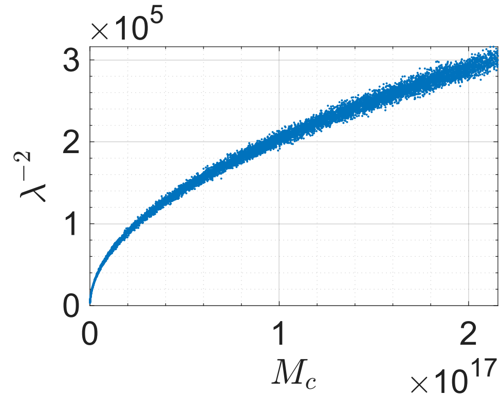
NGC6015 ( R_{\text{max}} = 29.23\text{kpc} )
