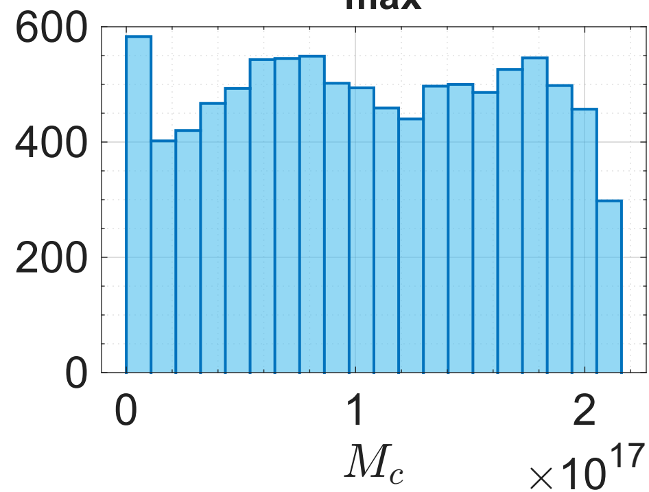
NGC6015 ( R_{\text{max}} = 29.23\text{kpc} )
