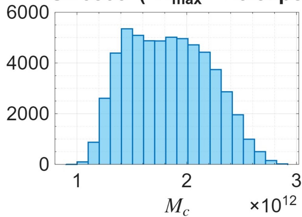
NGC6503 ( R_{\text{max}} = 23.5\text{kpc} )
