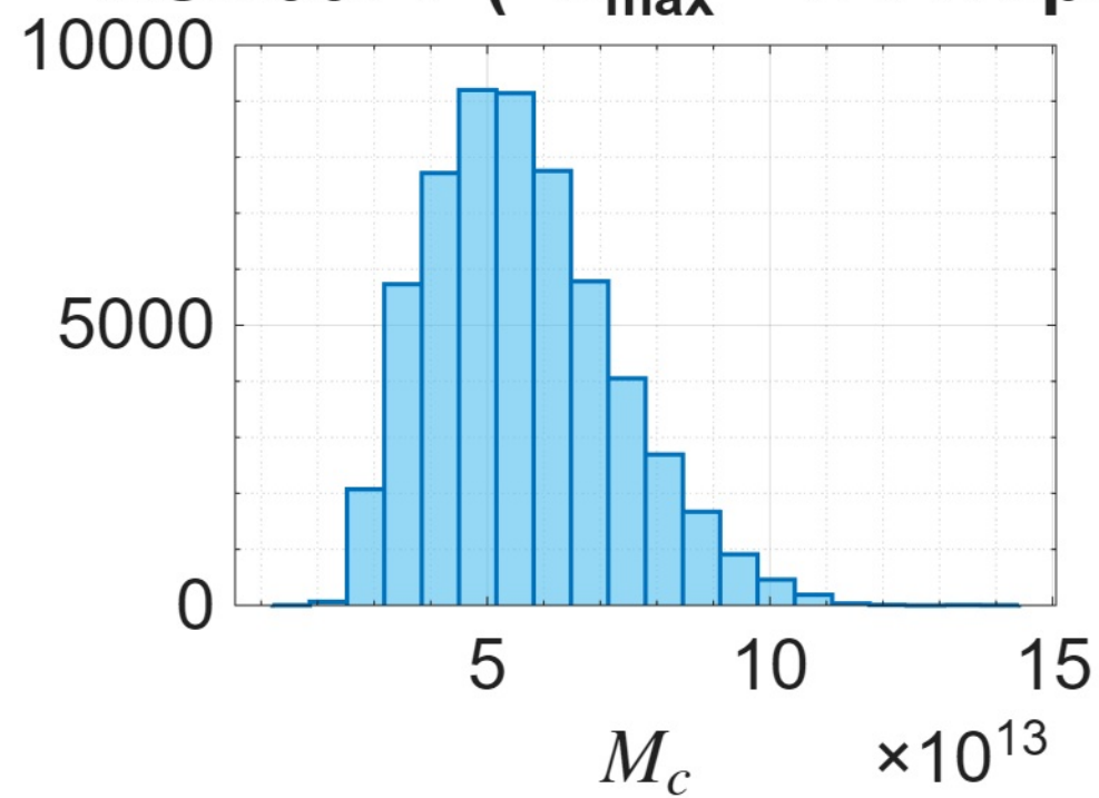
NGC6674 ( R_{\text{max}} = 72.41\text{kpc} )
