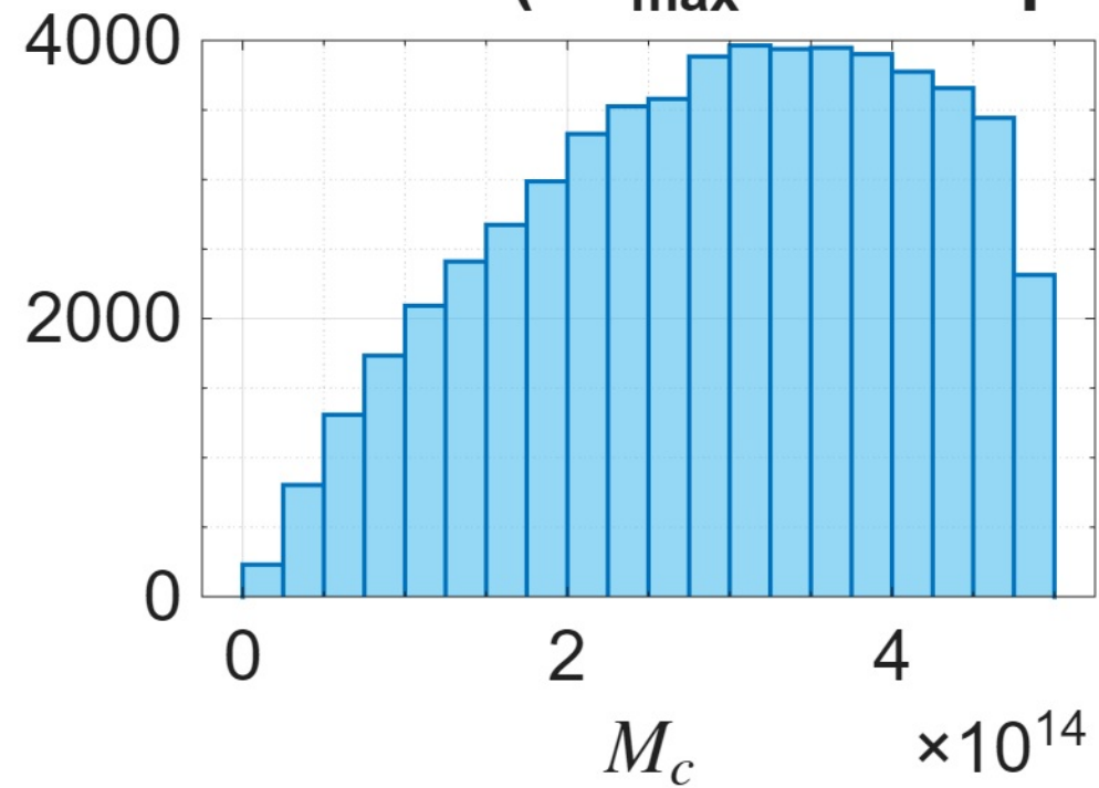
NGC6789 ( R_{\text{max}} = 0.71\text{kpc} )
