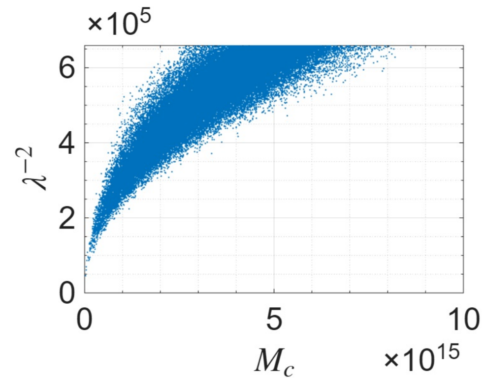
NGC7331 ( R_{\text{max}} = 36.31\text{kpc} )
