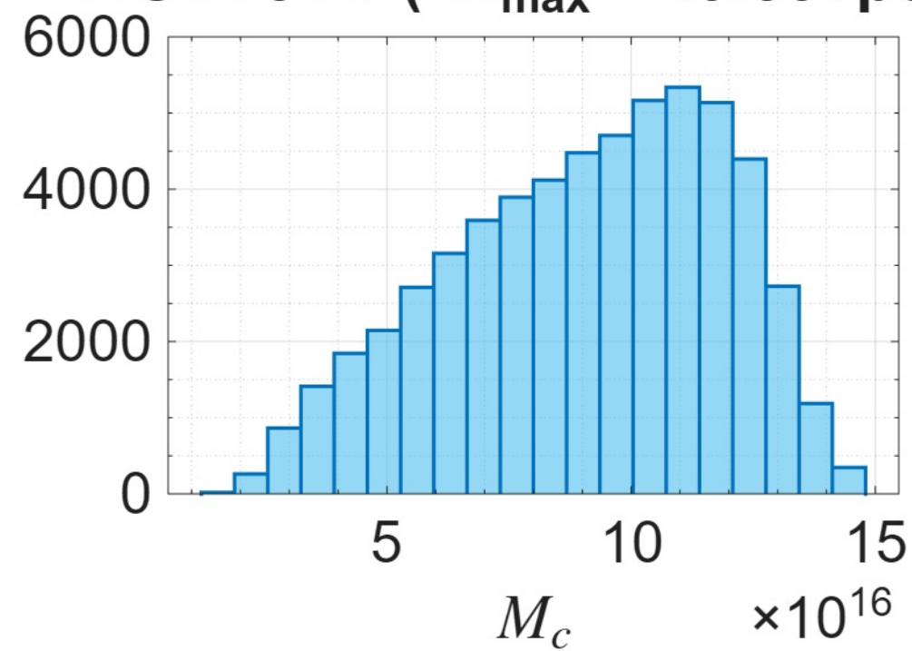
NGC7814 ( R_{\text{max}} = 19.53\text{kpc} )
