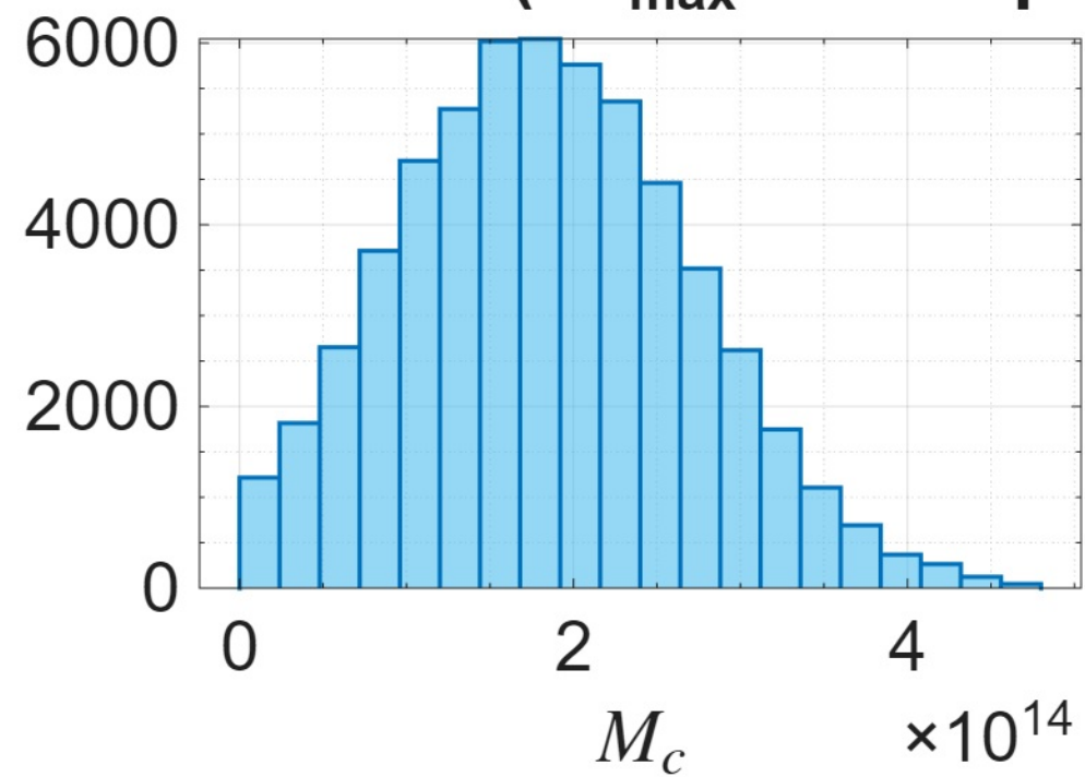
UGCA281 ( R_{\text{max}} = 1.08\text{kpc} )
