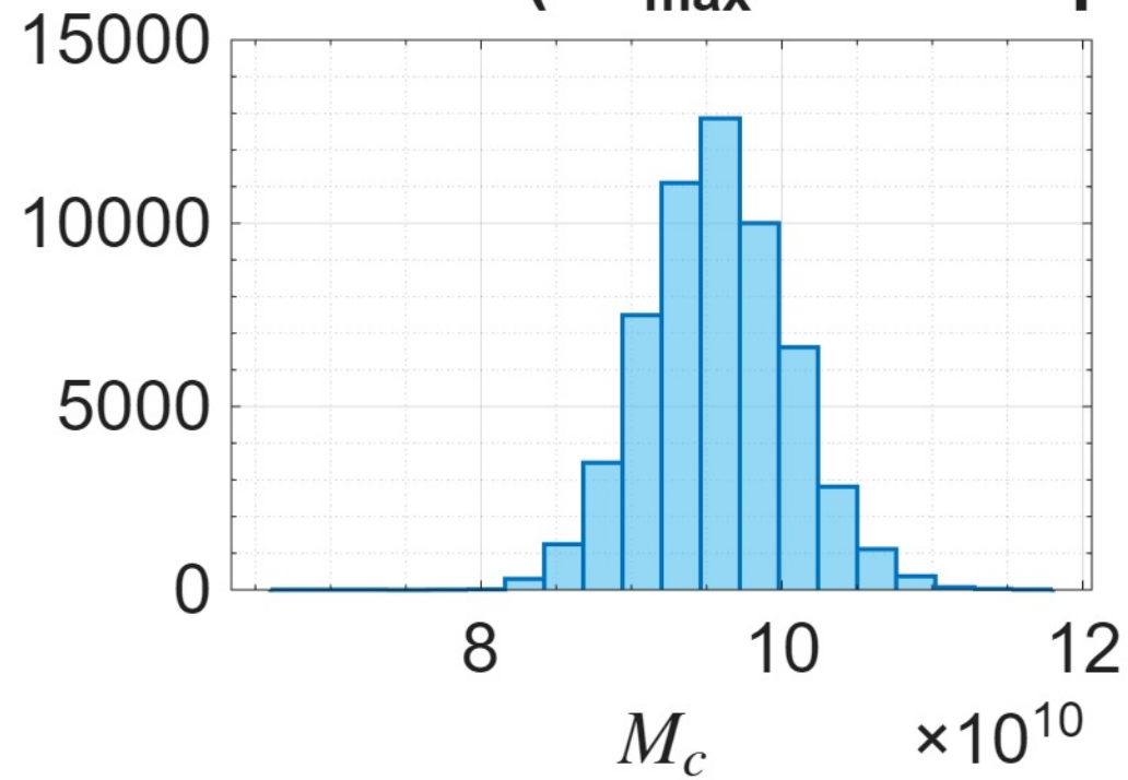
UGC00731 ( R_{\text{max}} = 10.91\text{kpc} )
