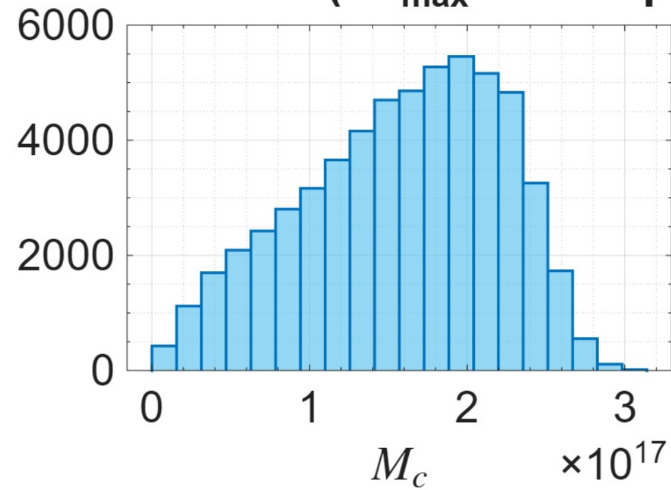
UGC08699 ( R_{\text{max}} = 25.7\text{kpc} )
