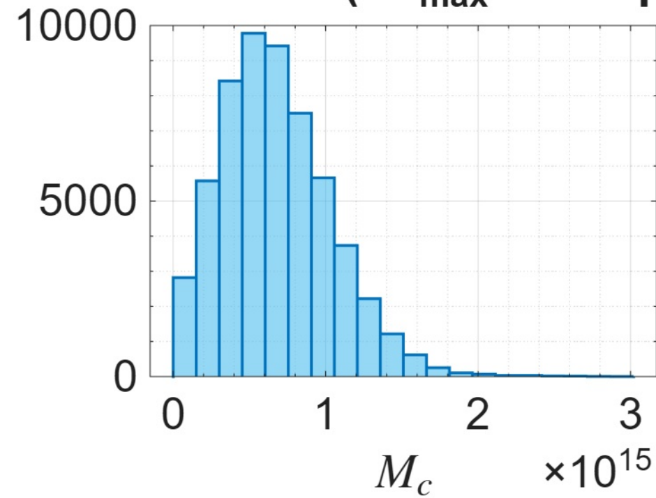
UGC08837 ( R_{\text{max}} = 4.2\text{kpc} )
