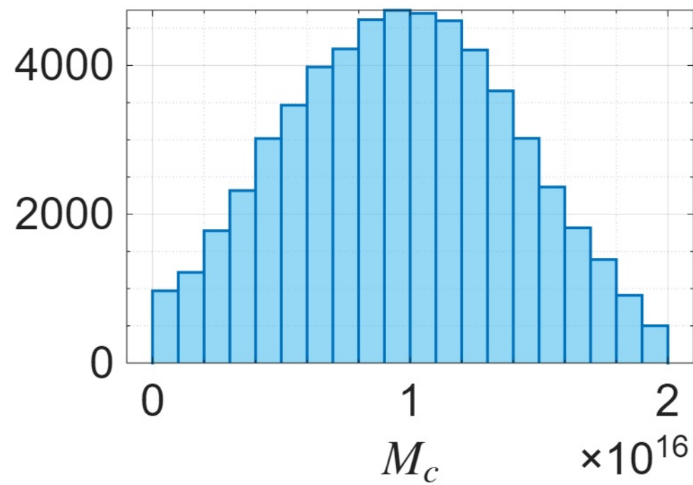
UGC10310 ( R_{\text{max}} = 7.74\text{kpc} )
