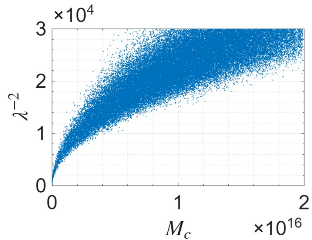
UGC10310 ( R_{\text{max}} = 7.74\text{kpc} )
