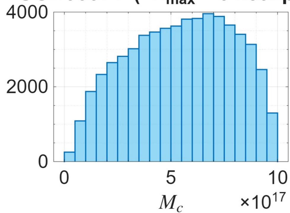
UGC06614 ( R_{\text{max}} = 64.59\text{kpc} )
