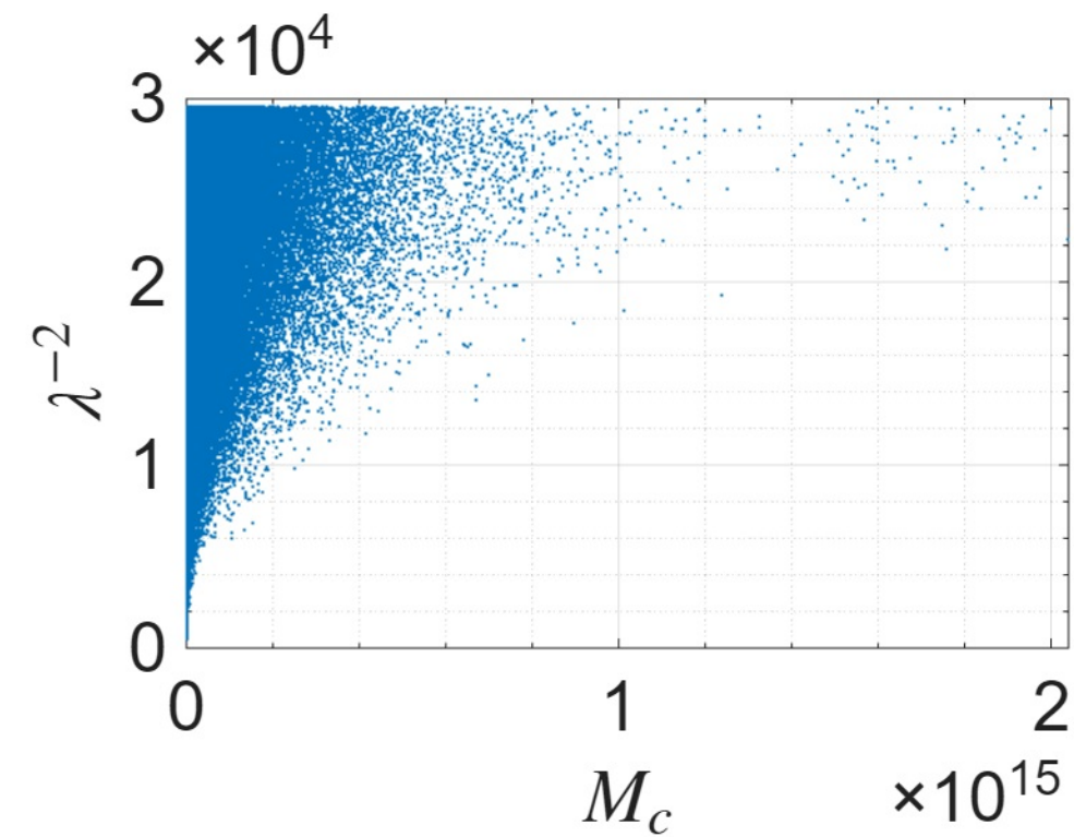
UGC06628 ( R_{\text{max}} = 7.69\text{kpc} )
