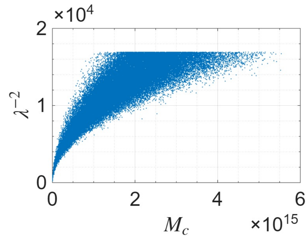
UGC07323 ( R_{\text{max}} = 5.82\text{kpc} )
