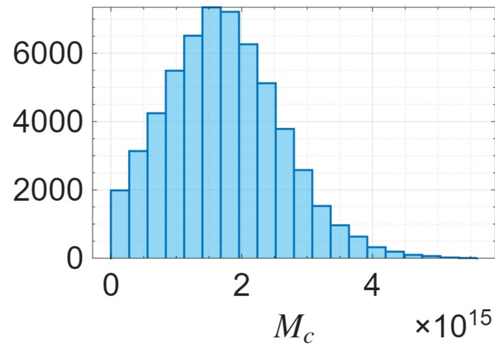
UGC07323 ( R_{\text{max}} = 5.82\text{kpc} )
