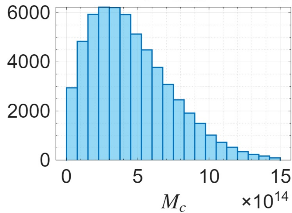
UGC07559 ( R_{\text{max}} = 2.53\text{kpc} )
