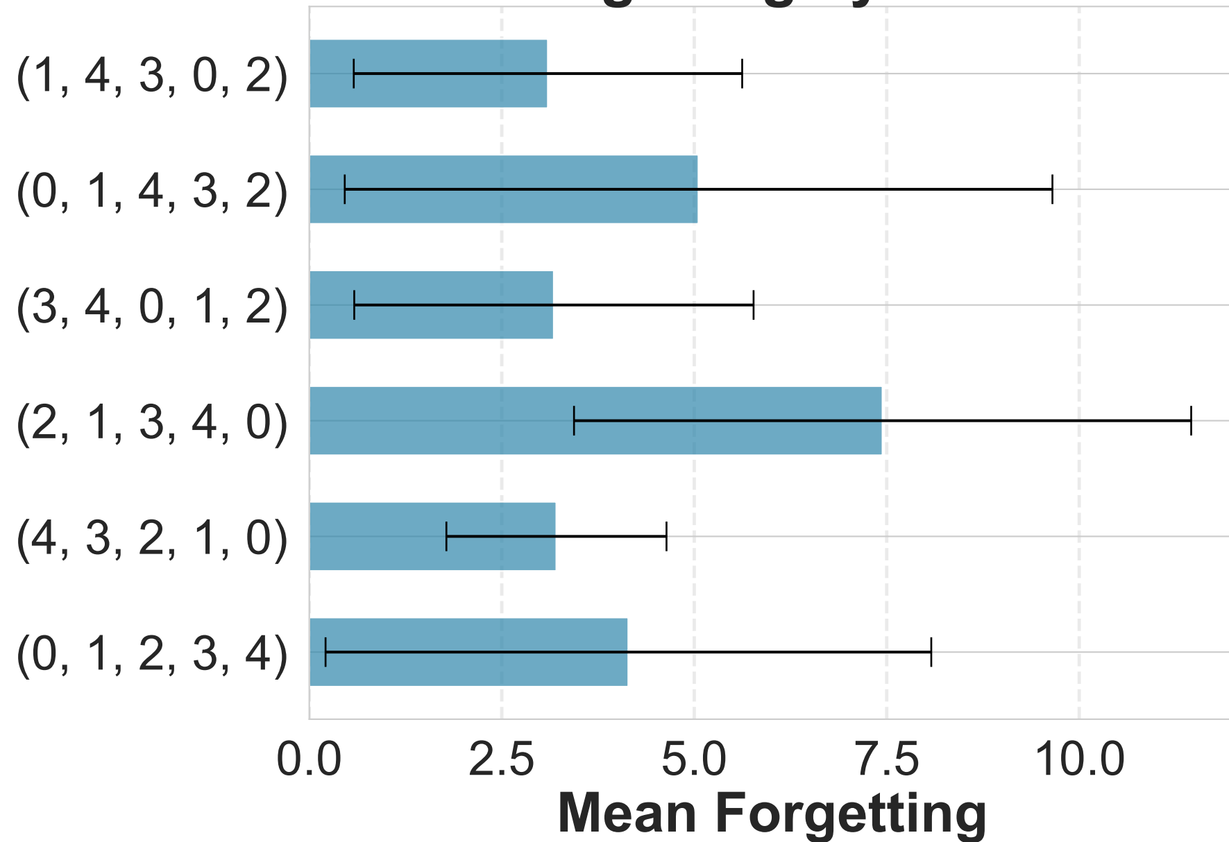
Mean Forgetting by Task Order
