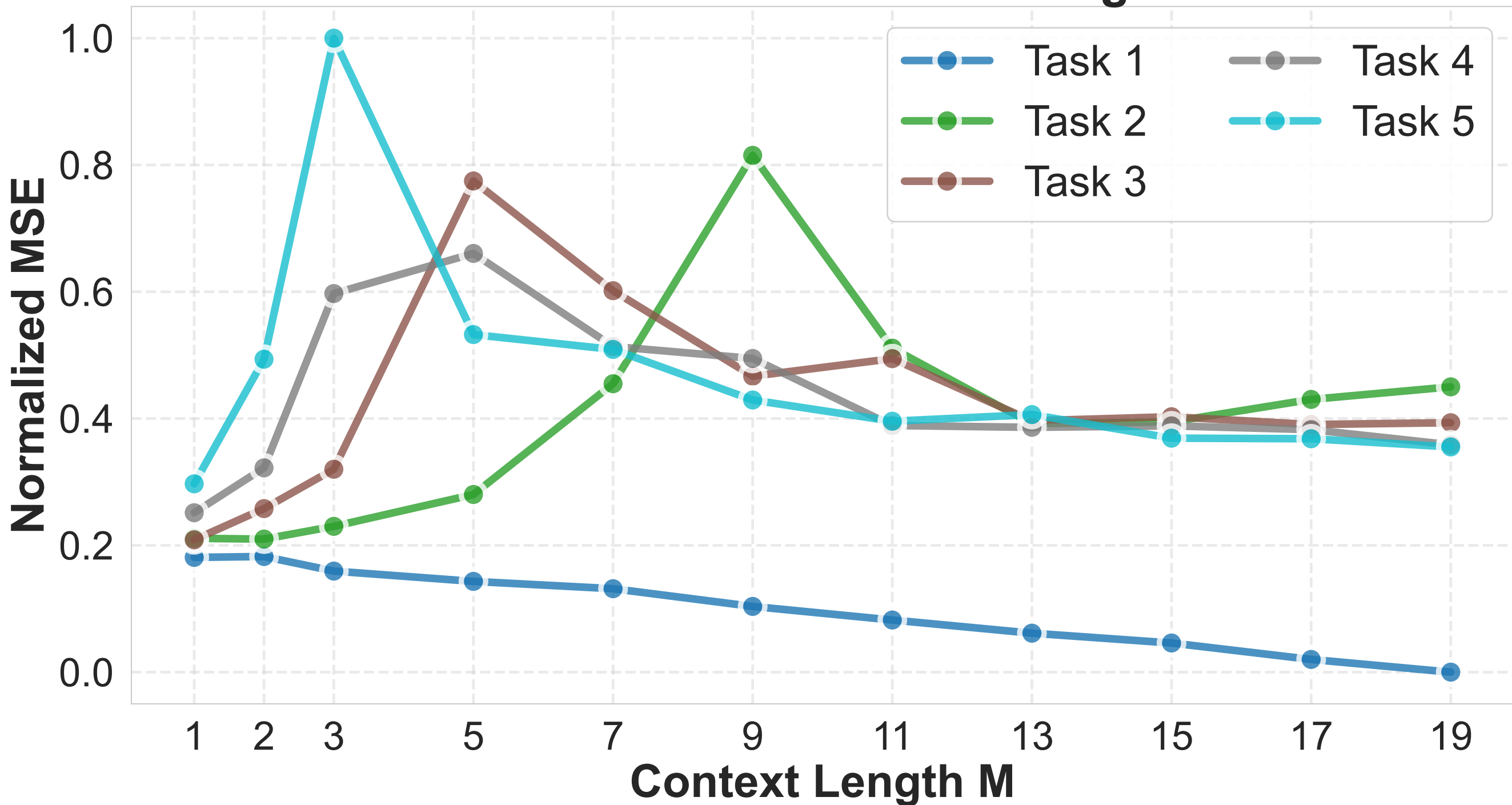
Per-Task MSE vs Context Length M
