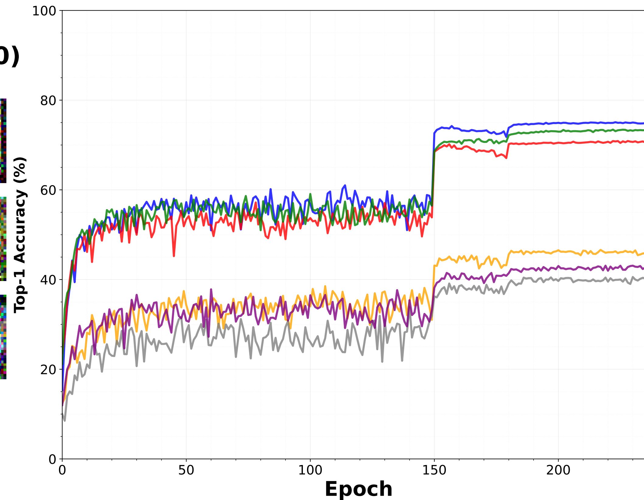
(b) Top-1 Accuracy
