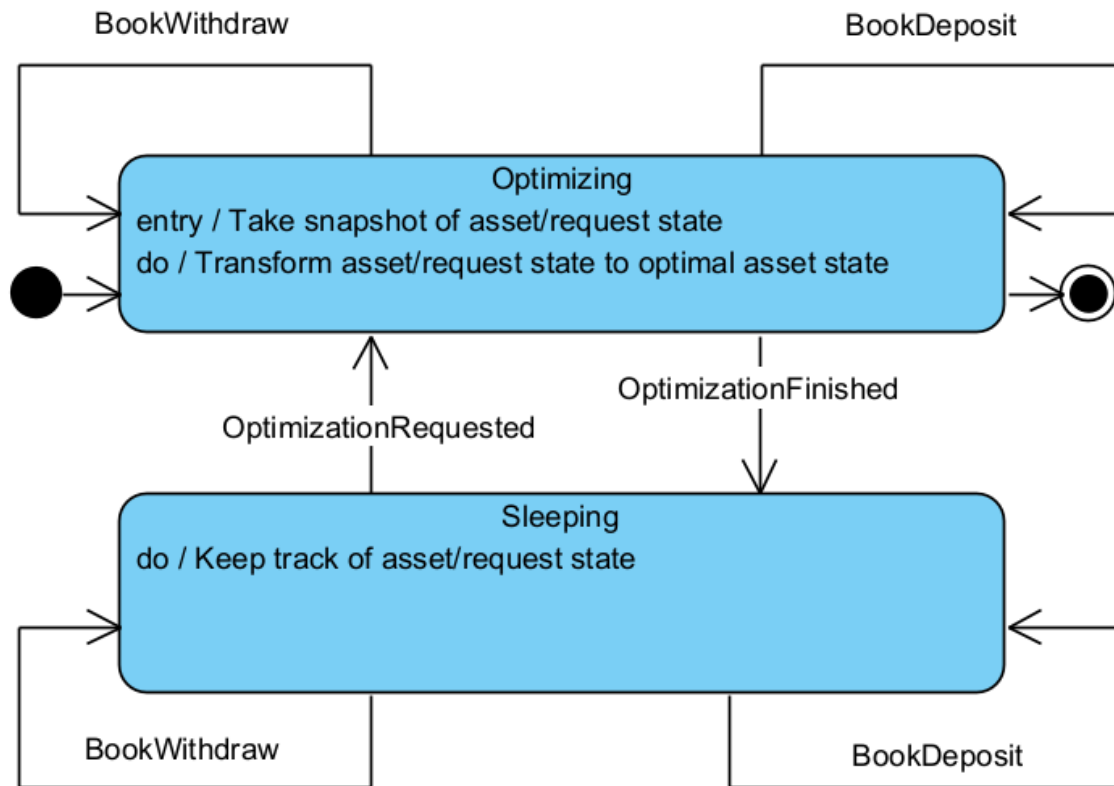
Figure. State Machine of Mozaic asset management
