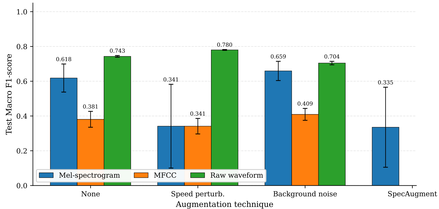
Phase 1: Preprocessing × Augmentation (CNN+GRU)
