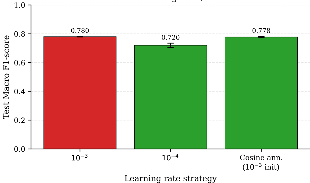
Phase 2b: Learning rate / scheduler
