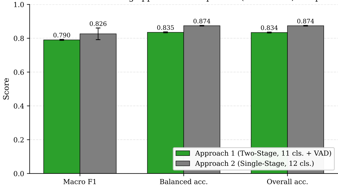
Phase 3: Silence handling approaches comparison (CNN+GRU, 30 epochs)
