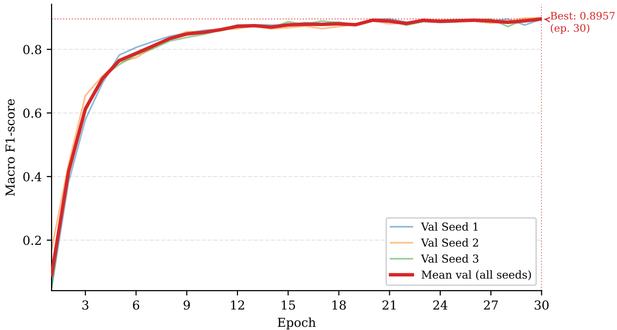
CNN+GRU Two-Stage: validation Macro F1 per epoch (30 epochs)
