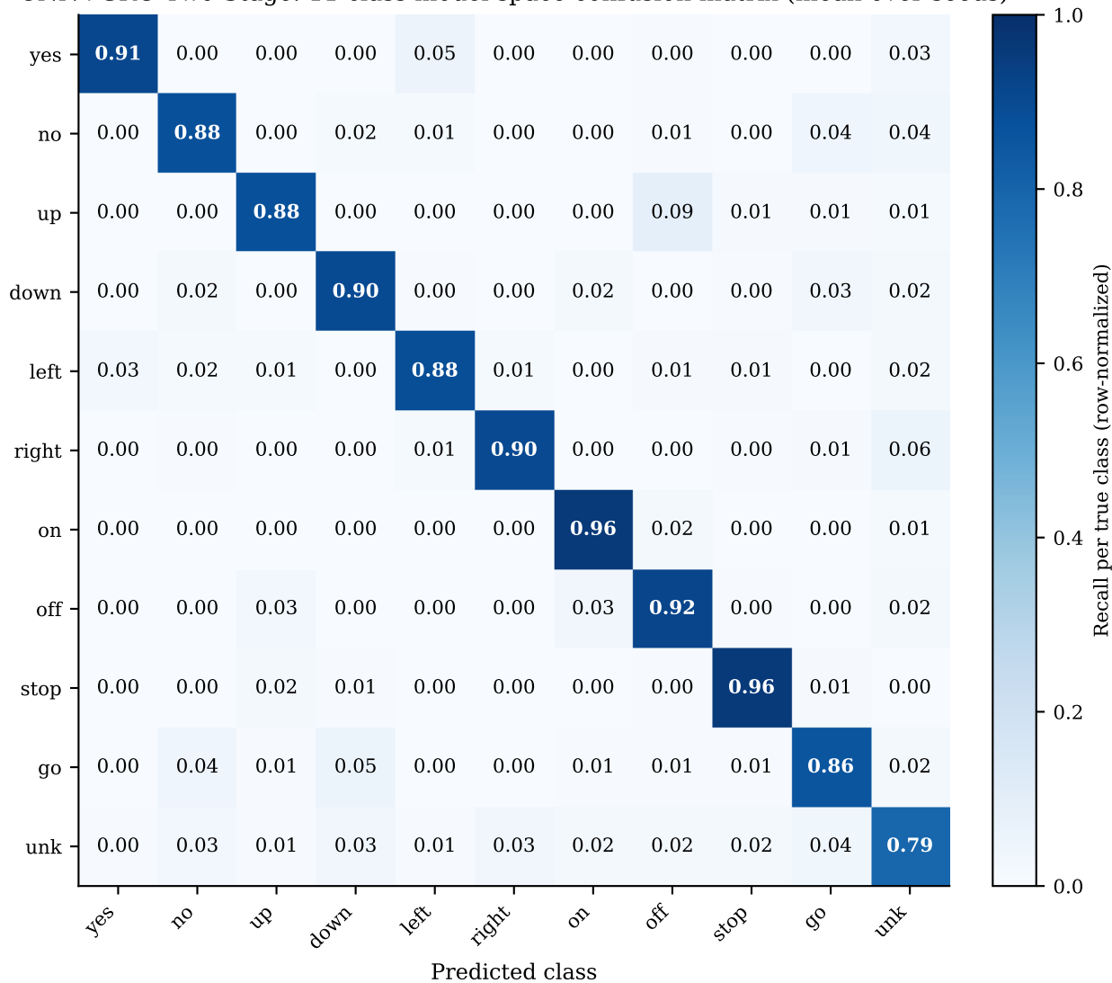
CNN+GRU Two-Stage: 11-class model space confusion matrix (mean over seeds)
