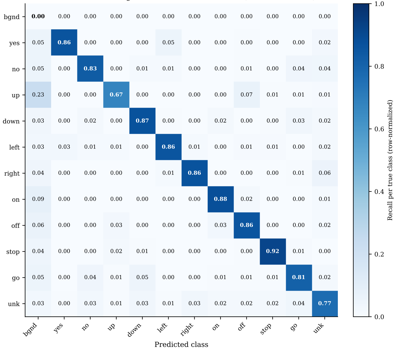
CNN+GRU Two-Stage: 12-class confusion matrix (mean over seeds)
