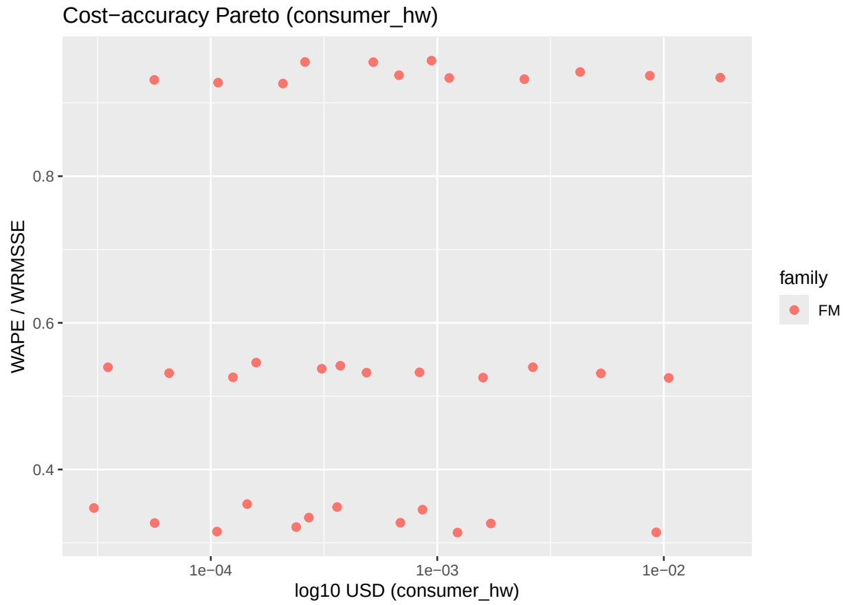
Figure 6: Cost-accuracy Pareto frontier on consumer hardware. X-axis: \log_{10} USD marginal electricity cost. Y-axis: best WAPE/WRMSSE. The four Source B FMs span the 9 M–120 M parameter range.
