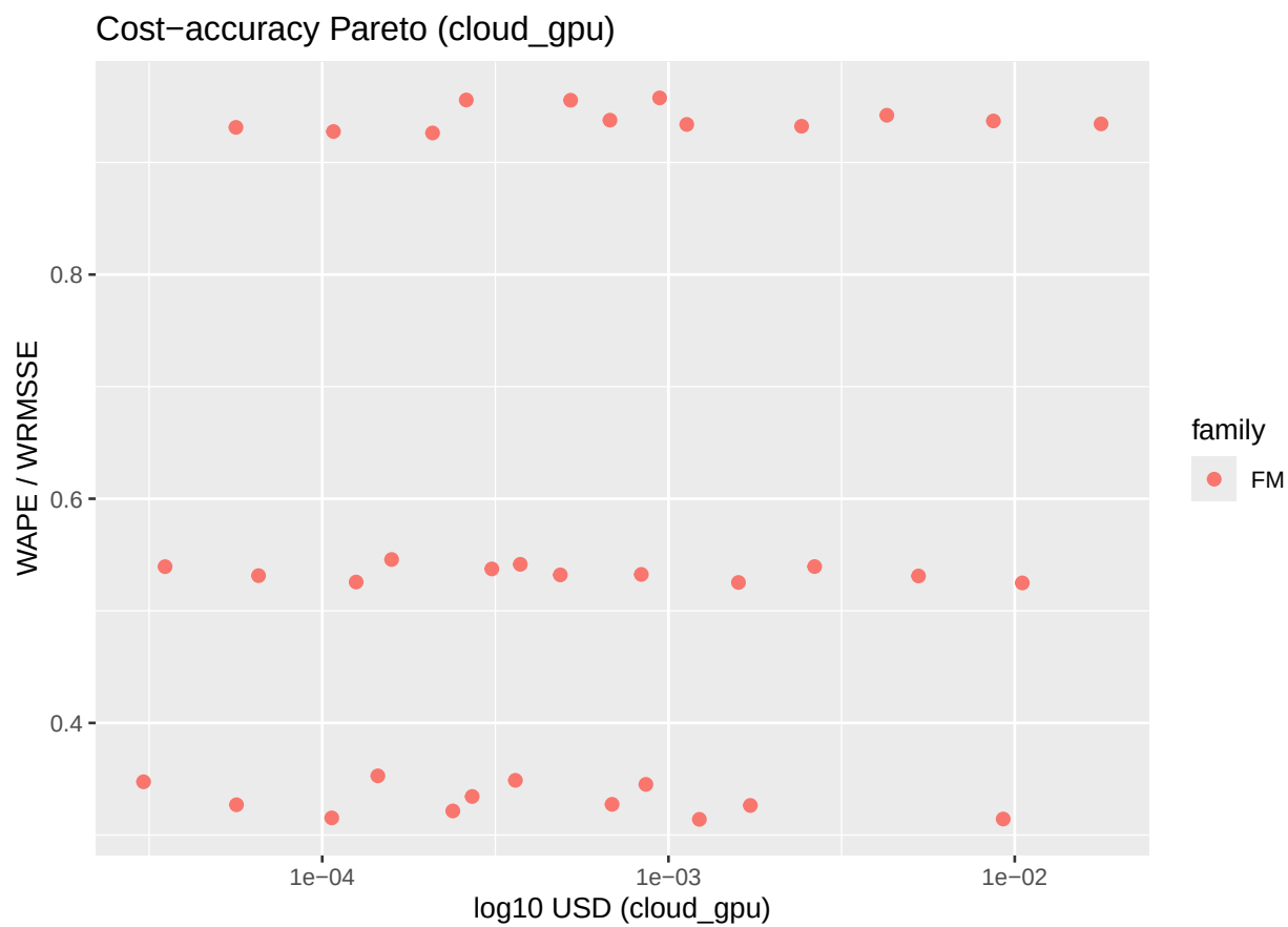
Figure 7: Cost-accuracy Pareto frontier re-costed on cloud GPU (V100 at $1.24/hr).
