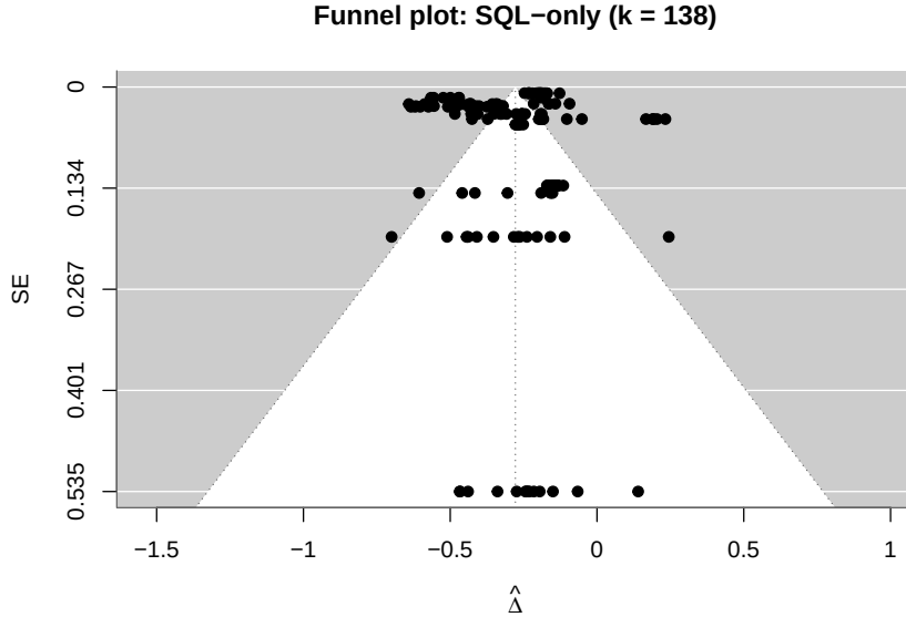
Figure 6: Funnel plot for SQL-only slice ( k = 138 ). No evidence of asymmetry (Egger-type test p = 0.46 ).
