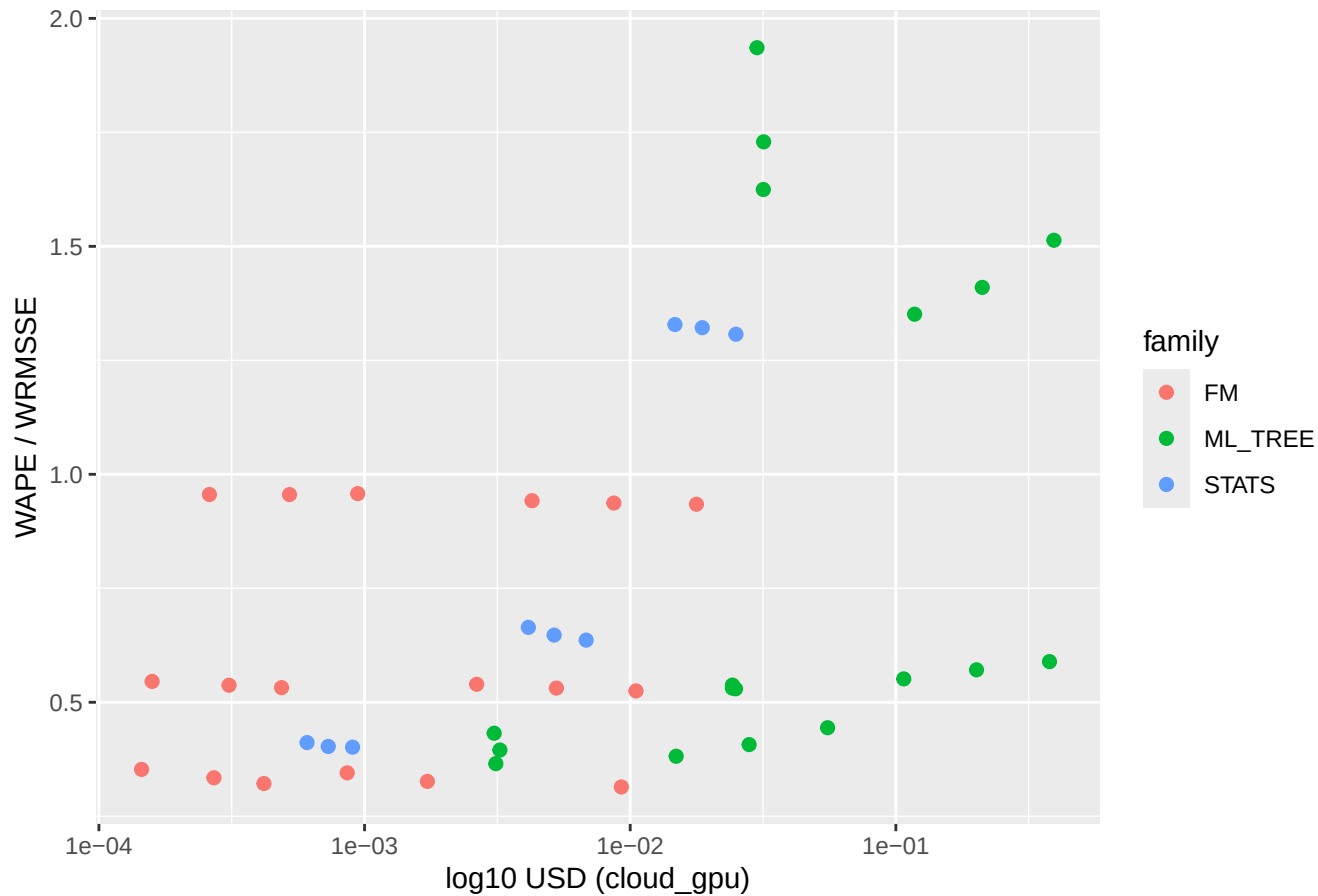
Cost-accuracy Pareto (cloud_gpu)
