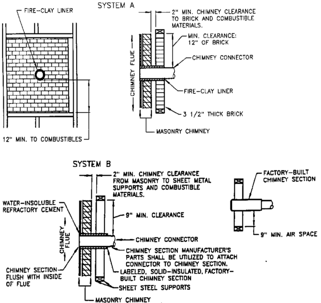
FIGURE A-1 CHIMNEY CONNECTOR SYSTEMS
