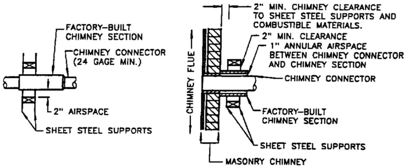
FIGURE A-1—continued CHIMNEY CONNECTOR SYSTEMS
