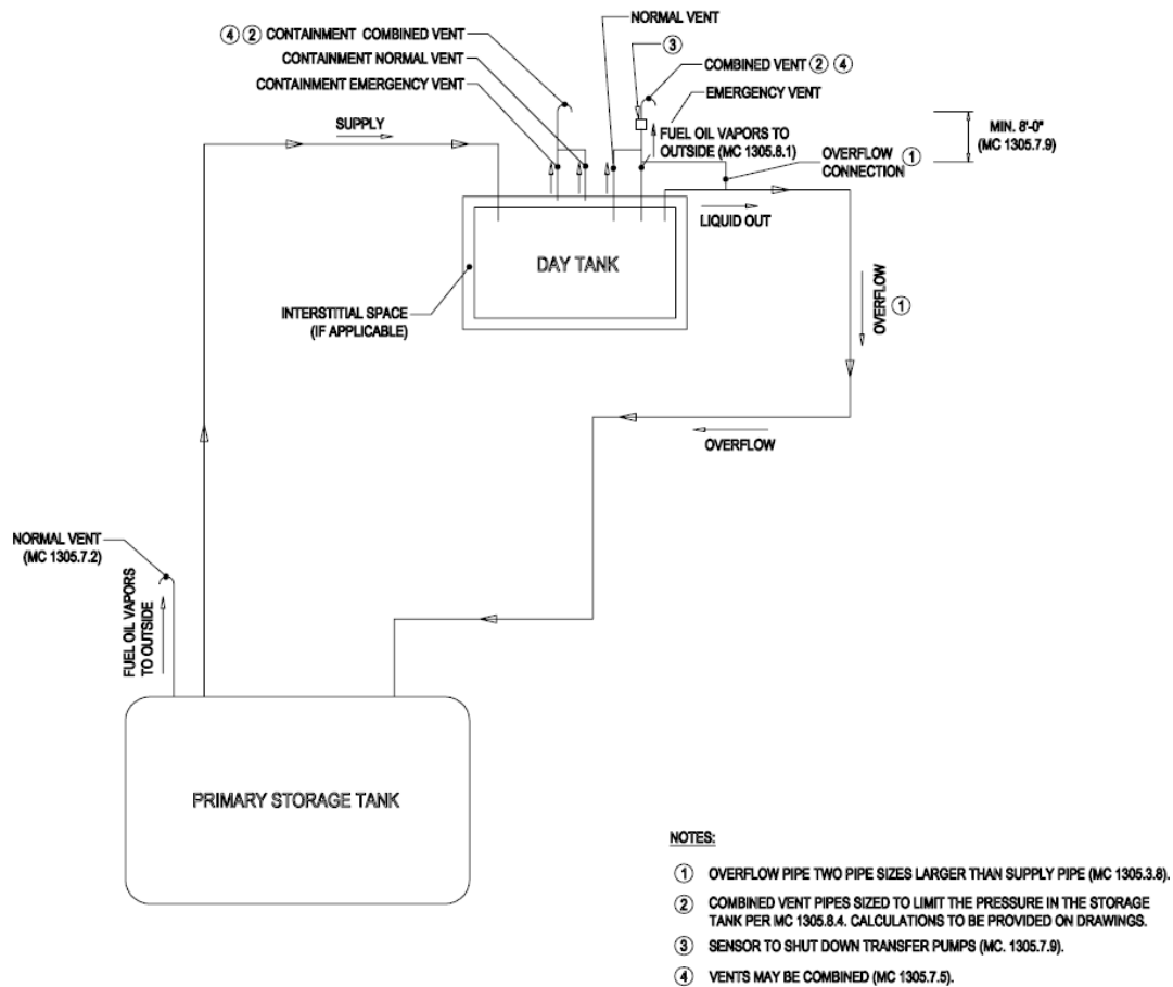
FIGURE C101.1(3) PRIMARY TANK: UL 80, ASME BPVC, OR NYC ALTERNATE TANK DAY TANK: UL 142 OR DUAL LABEL TANK
