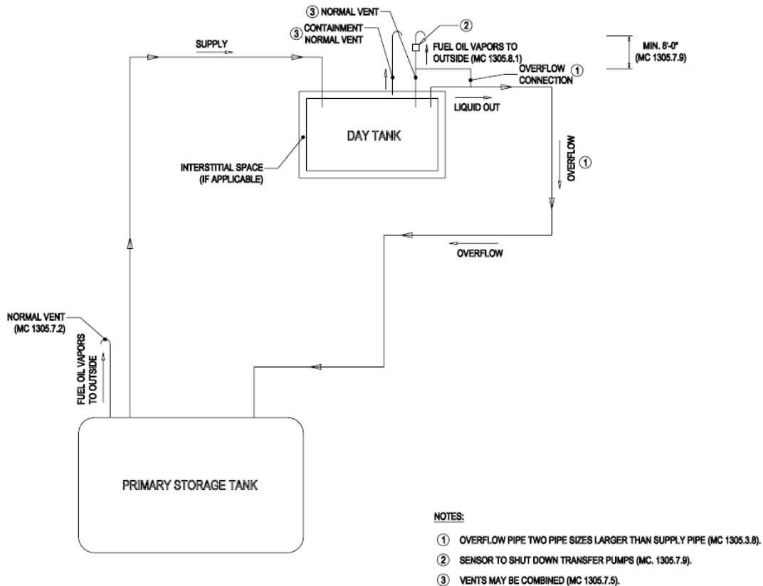
FIGURE C101.1(1) PRIMARY TANK: UL 80, ASME BPVC, OR NYC ALTERNATE TANK DAY TANK: UL 80, ASME BPVC, OR NYC ALTERNATE TANK
