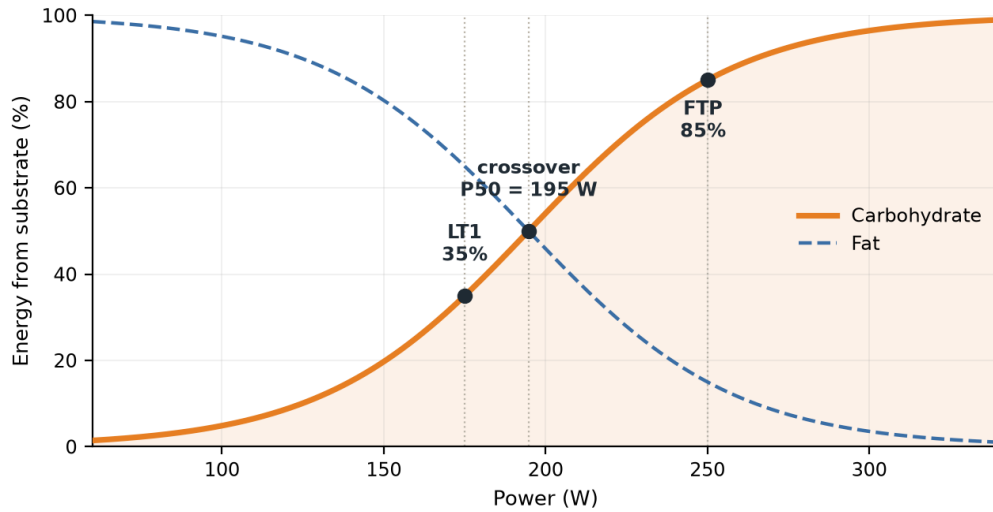
Figure 1. Modelled substrate split for a generic sample rider (FTP = 250 W, LT1 estimated at 175 W, GE = 0.21). The carbohydrate fraction f(P) follows the logistic curve anchored at 35% at LT1 and 85% at FTP; fat supplies the remainder. The crossover point (50% carbohydrate) falls at P_{50} \approx 195 W.
