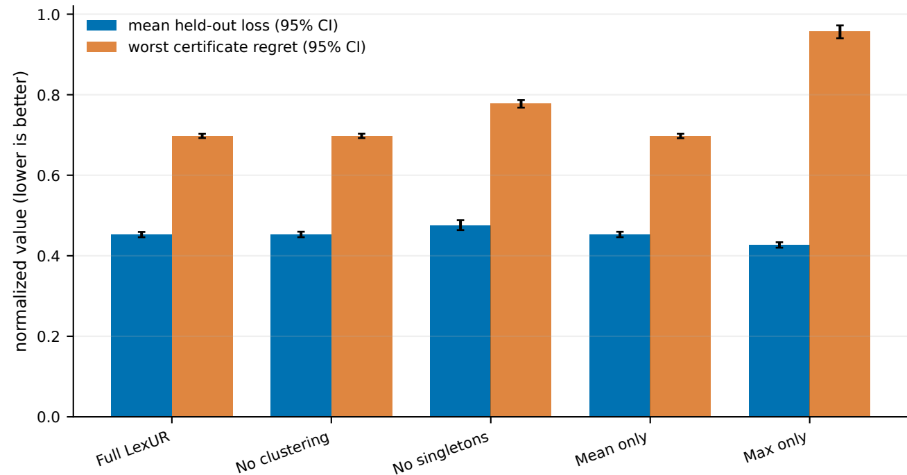
Probe-family ablations, including null results
