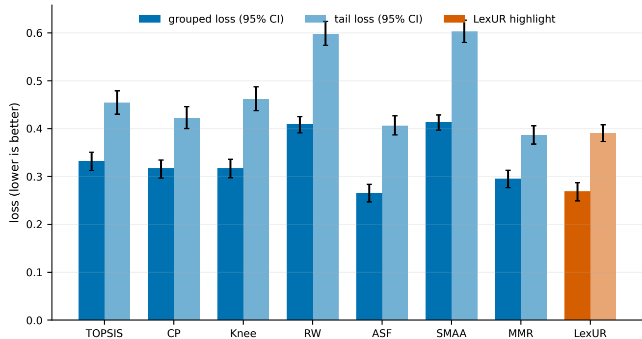
Robustness to redundant criteria
