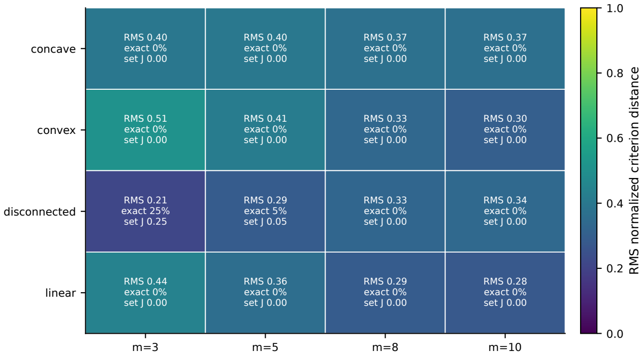
LexUR versus SMAA recommendations
