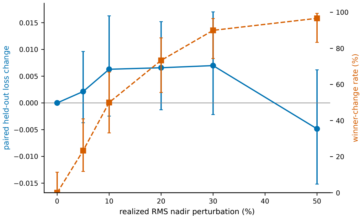
Nadir sensitivity: quality and identity are paired diagnostics
