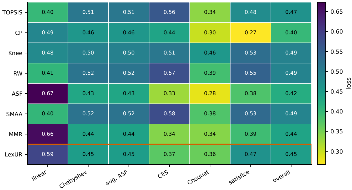
Held-out loss by preference family (concave, m = 8 ; lower is better)
