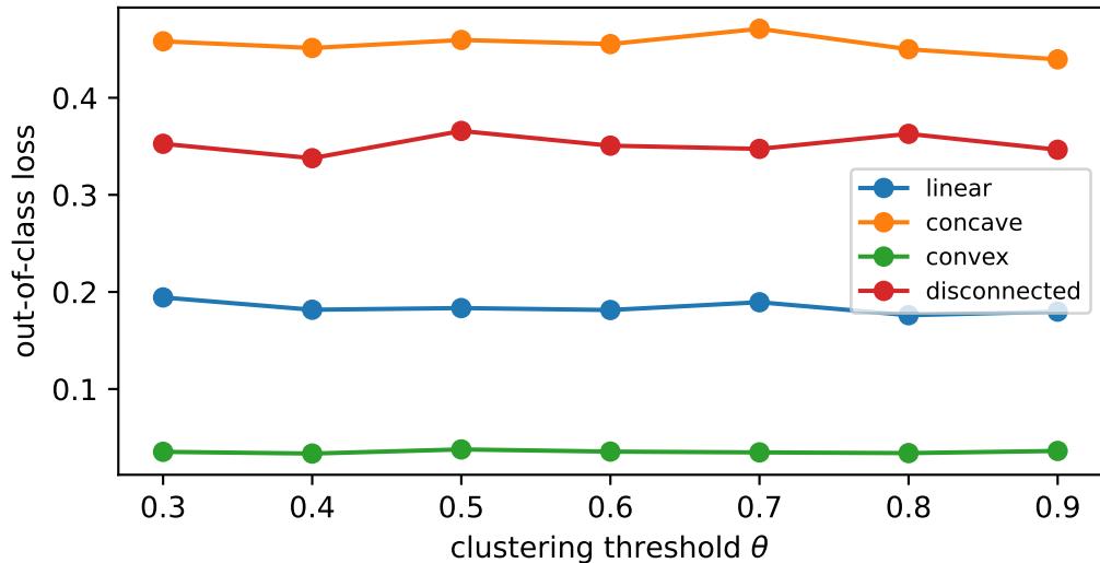
LUR sensitivity to \theta across geometries (m=8)
